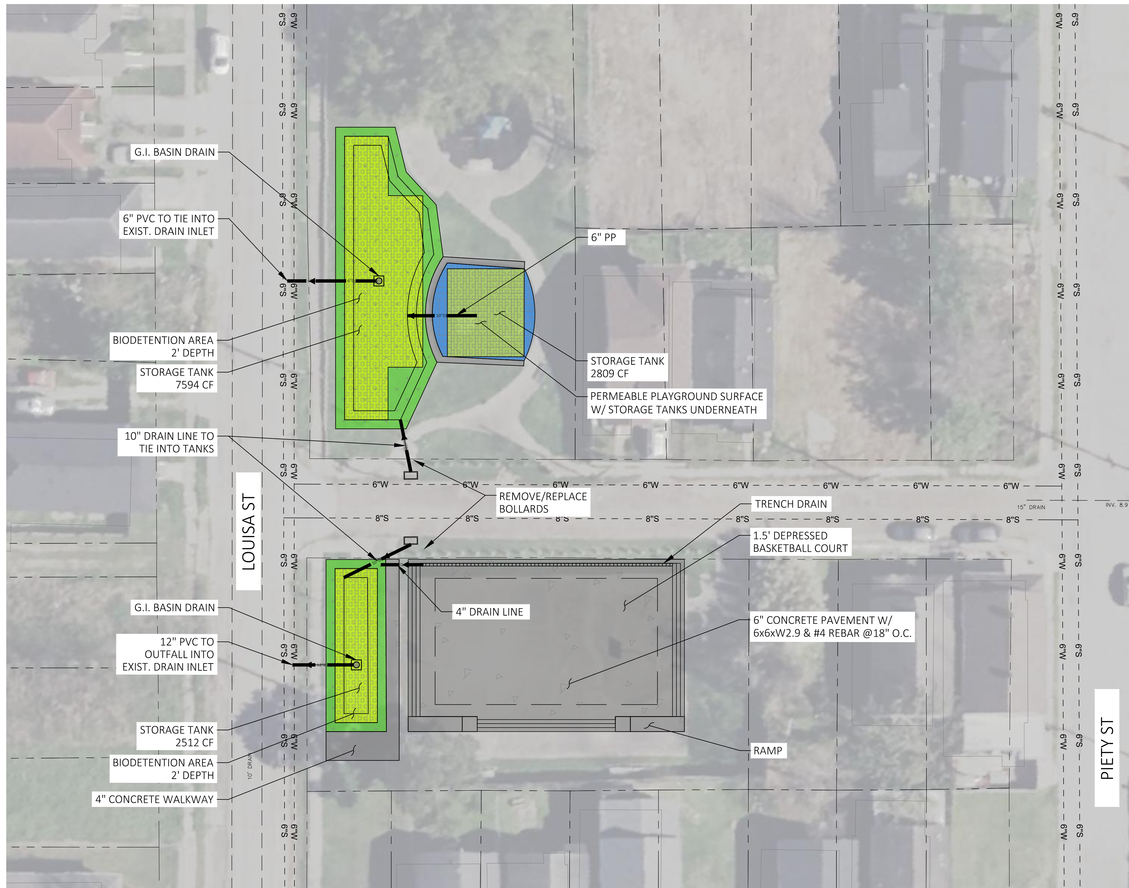
C1 CONCEPTUAL SITE PLAN - PROJECT G
